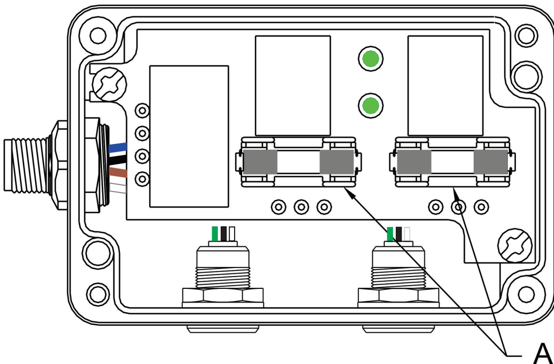
Figure 3: Relay Output Replaceable Fuse Location
