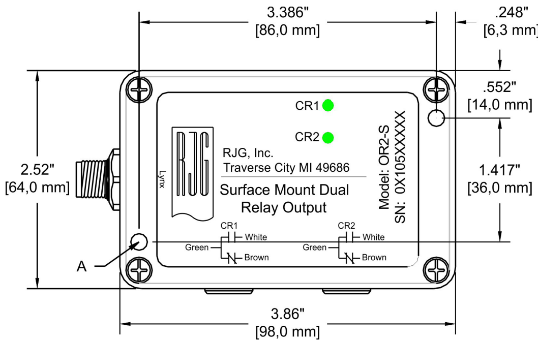
Figure 1: Lynx™ Dual Relay Output Module - OR2-S
