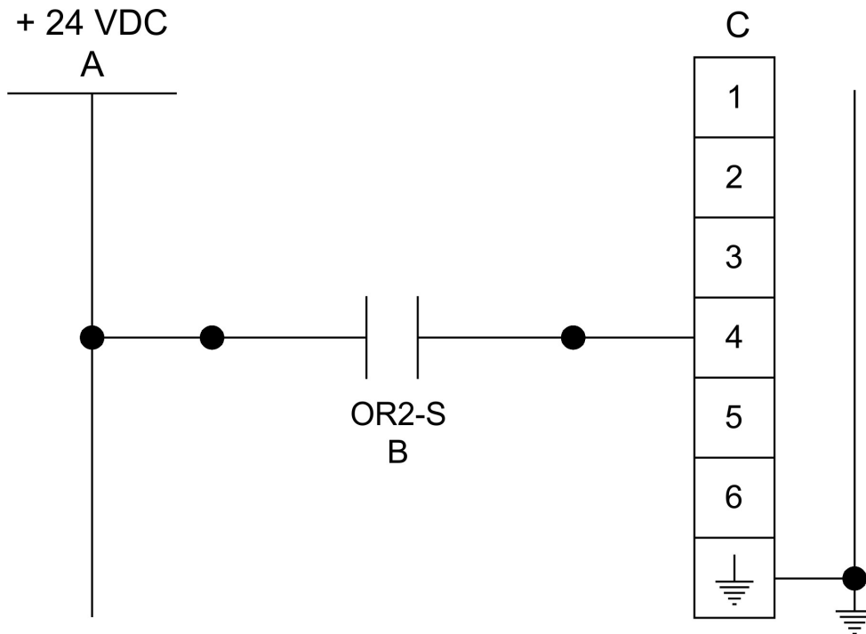
Figure 2: Lynx™ Dual Relay Output Module Interface with one type of Robot Interface
